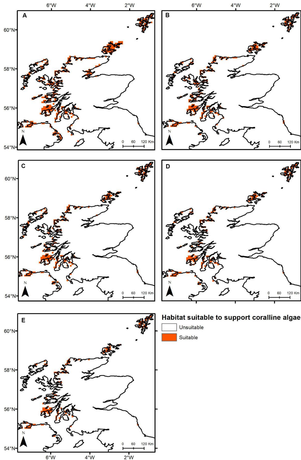
Figure 26. Threshold maps of coralline algal beds distribution around Scotland in the present-day (A) and by 2100 under the IPCC Representative Concentration Pathway (RCP) emission scenarios. (B) RCP 2.6, (C) RCP 4.5, (D) RCP 6.0, and (E) RCP 8.5. Orange indicates predicted presence of coralline algal beds. Source: Simon-Nutbrown et al. (2020), available under a Creative Commons BY license ( CC BY 4.0 ), no changes made.
