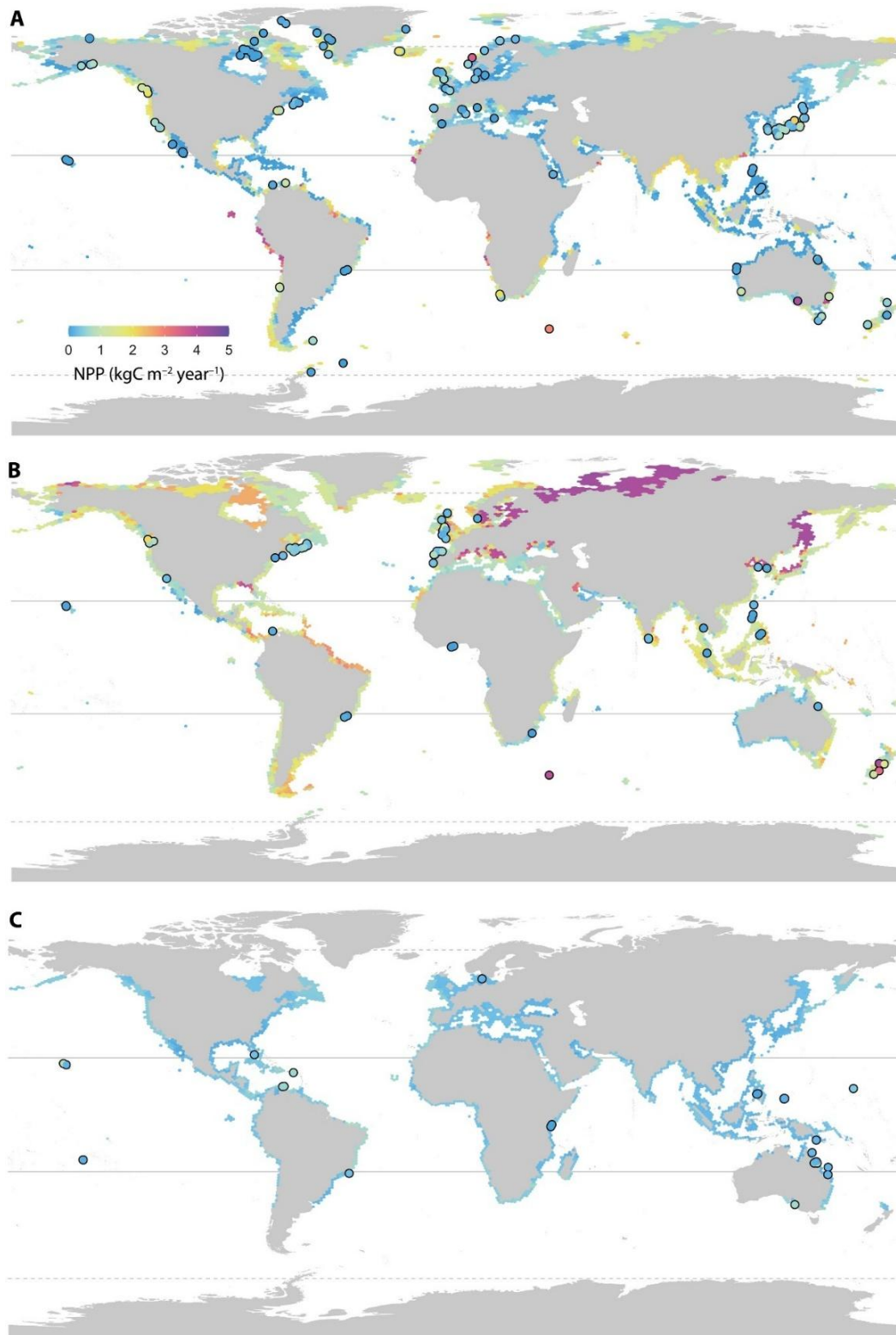
Figure 4. Globally predicted net primary productivity (NPP) of subtidal (A) and intertidal (B) seaweed forests dominated by large brown canopy-forming algae and (C) subtidal algal turfs. Points show the location of the study sites included in this database (raw NPP is indicated by the coloured dots). Lines depict the tropics (straight) and polar circles (dashed). Source: Pessarodona et al. (2022), available under a Creative Commons Attribution License 4.0 ( CC BY 4.0 ).
