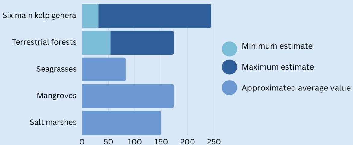
Figure 7. Estimated carbon sequestration rates ( \text{g m}^{-2} \text{ year}^{-1} ) for six main kelp genera compared to other vegetated habitats. Adapted from Eger et al., 2023a. Sources: Eger et al., (2023) (kelp), Toohey et al., (2018) (terrestrial forests), Laffoley & Grimsditch (2009) (seagrasses), Alongi (2012) (mangroves and saltmarshes).
