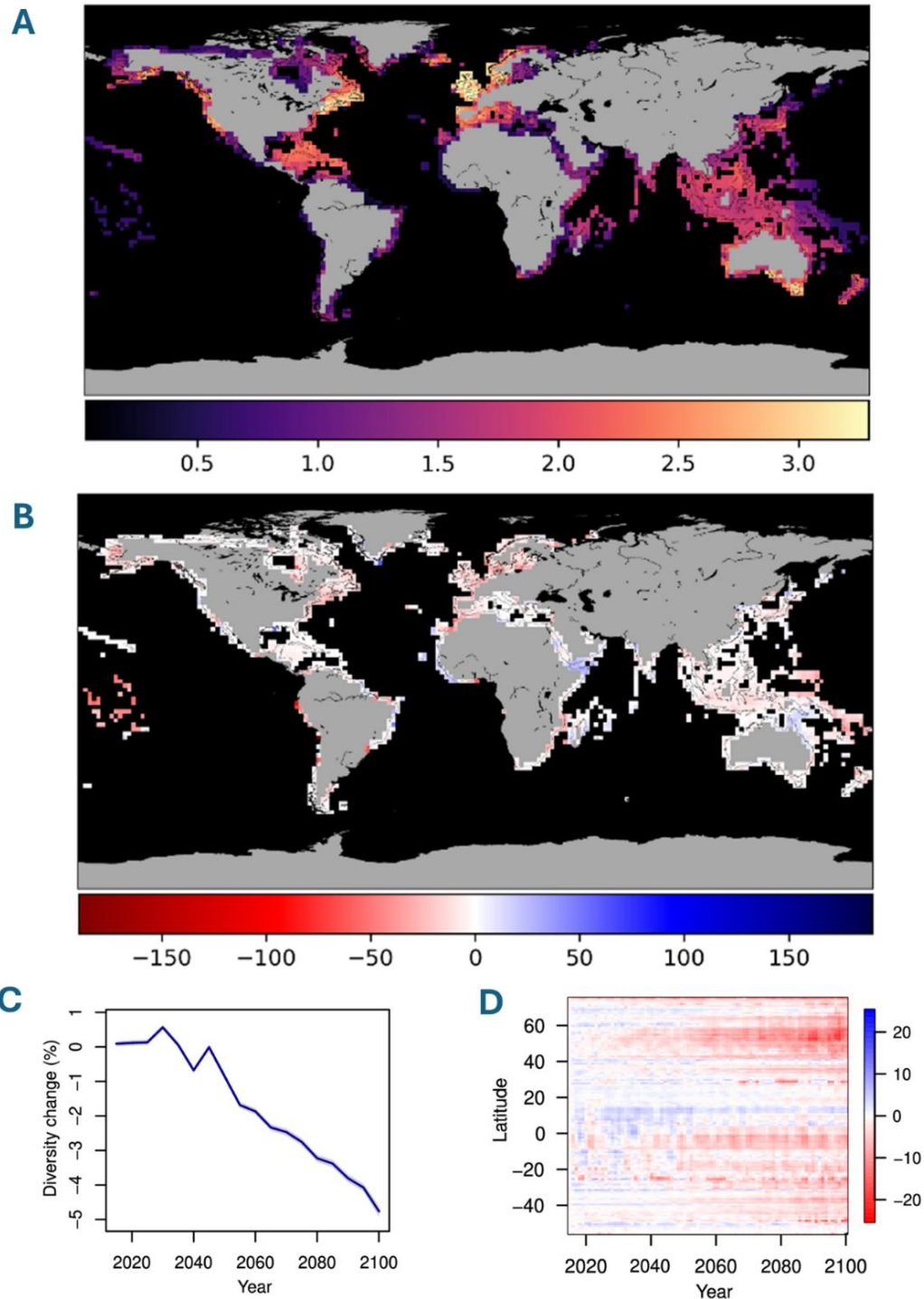
Figure 23. A. Present distribution. B. projected end-of-century changes in global brown macroalgal species diversity under an intermediate emissions scenario (SSP3-7.0). C. Mean trajectories in local brown macroalgal diversity (i.e., number of macrophyte species in every 0.5^\circ \times 0.5^\circ latitude/longitude grid cell) relative to 2015 (data were aggregated at 5-year intervals). D. Expected future changes in diversity as loge percentage change relative to 2015 diversity averaged across latitudes ( 0.5^\circ \times 0.5^\circ latitude/longitude resolution). B and D: species diversity gains = blue, losses = red. Adapted from Manca et al., 2024, available under a Creative Commons Attribution License 4.0 ( CC BY 4.0 ), no changes were made to the figures, however they have been compiled into one panel.
