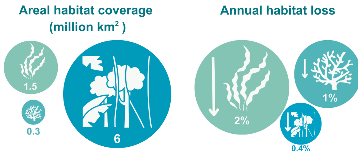
Figure 16. Global areal habitat coverage and annual habitat loss of kelp forests compared to the Amazon rainforest and coral reefs. Kelp forests cover an ocean area five times greater than all coral reefs and a quarter the size of the Amazon rainforest, however they are declining at an annual rate two times that of coral reefs and more than four times that of rainforests. Adapted from Feehan et al. (2021) and Filbee-Dexter et al. (2022b).
