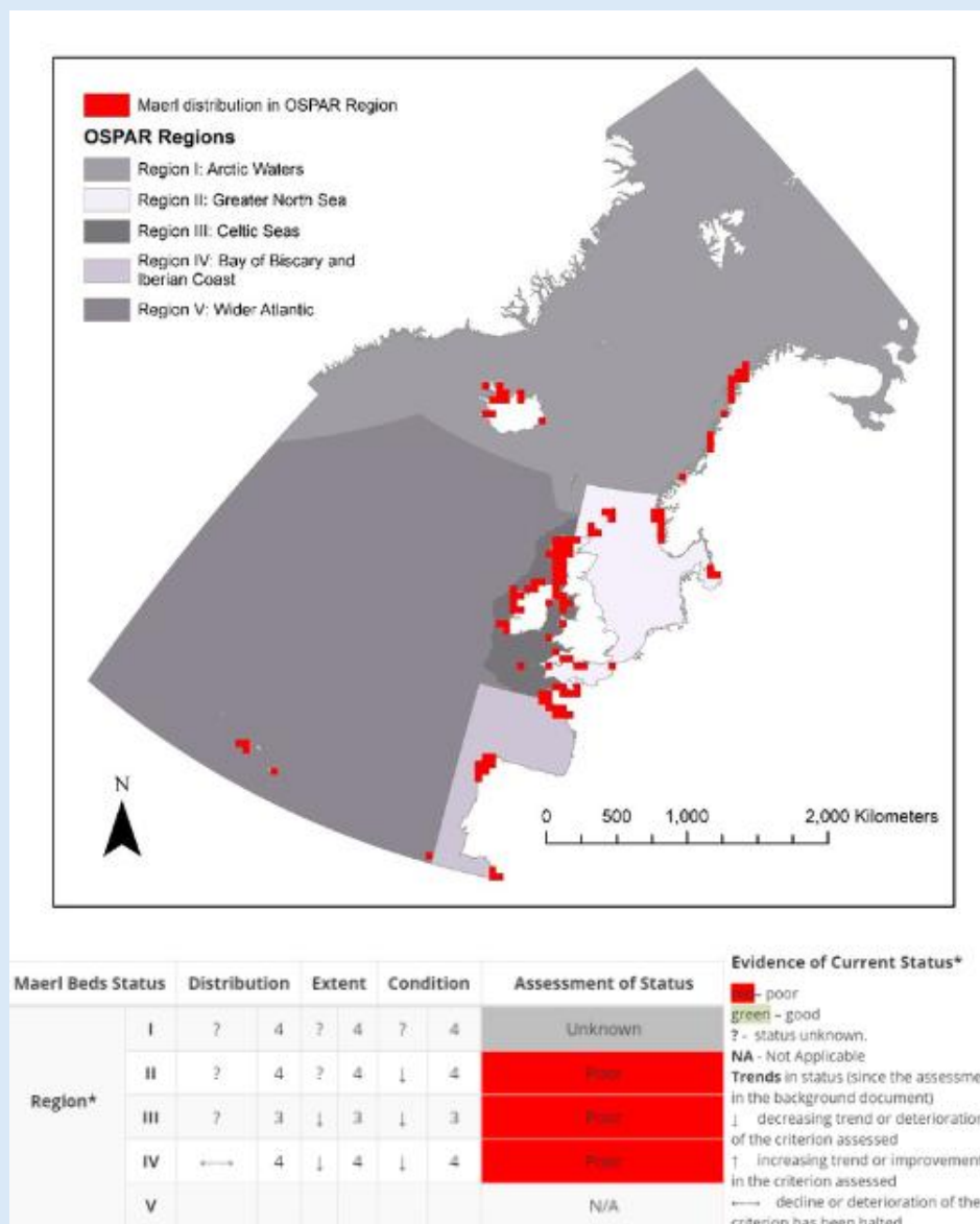
Figure 20. Distribution of 50 km squares containing maerl beds in the OSPAR maritime area, based on OSPAR T&D database (2018) and Article 17 data on Lithothamnion corallioides and Phymatolithon calcareum distribution from Spain. Source: OSPAR Commission (sheet reference: POSH2019/Maerl_Beds OSPAR ) available under a Creative Commons Attribution License 4.0 (CC BY 4.0).
