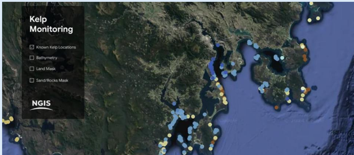
Figure 31. Example of the Google Earth Engine map showing known Giant Kelp locations in Tasmania. Source: Riddle, 2014 ( https://blog.google/intl/en-au/company-news/technology/ai-giant-kelp/ , accessed: 24/05/25).
