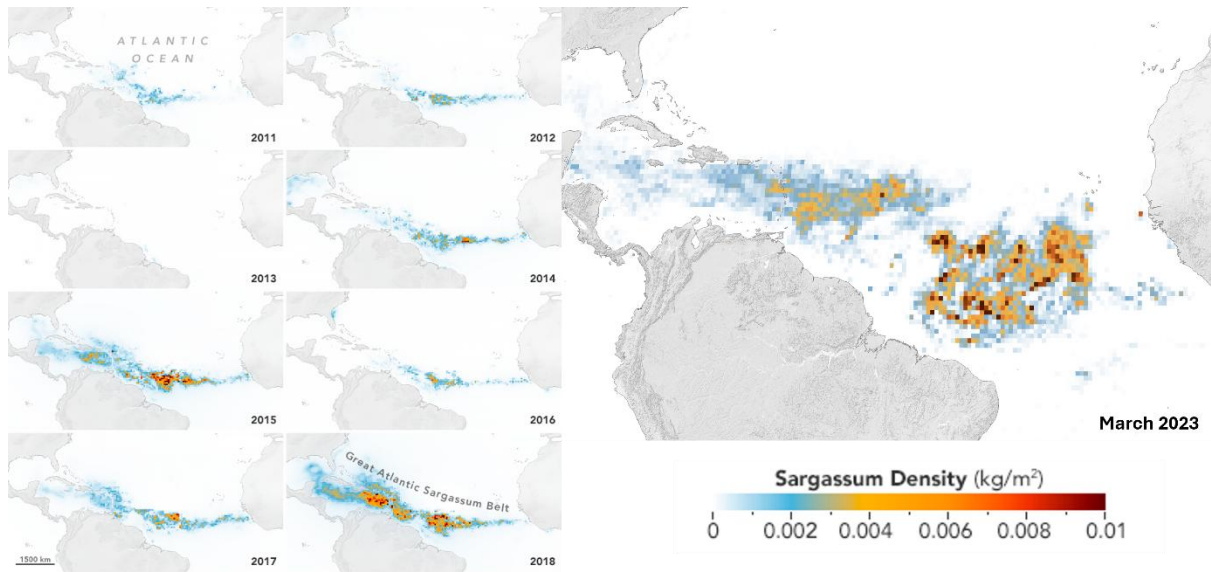
Figure 21. NASA Earth Observatory images of the “Great Atlantic Sargassum Belt” each year from 2011 to 2023 by Lauren Dauphin and Joshua Stevens, using MODIS satellite data courtesy of Brian Barnes at the University of South Florida (USF), Optical Oceanography Lab and Wang et al. (2019). Source: NASA, Available: https://earthobservatory.nasa.gov/images/151188/a-massive-seaweed-bloom-in-the-atlantic
