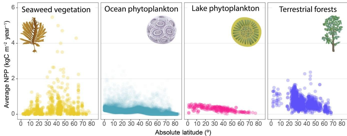
Figure 5. Relationship between latitude and net primary productivity (NPP) across Earth's major primary producers. Terrestrial forest NPP includes above and below ground productivity. Source: Pessarodona et al. (2022) available under a Creative Commons Attribution License 4.0 (CC BY 4.0).
