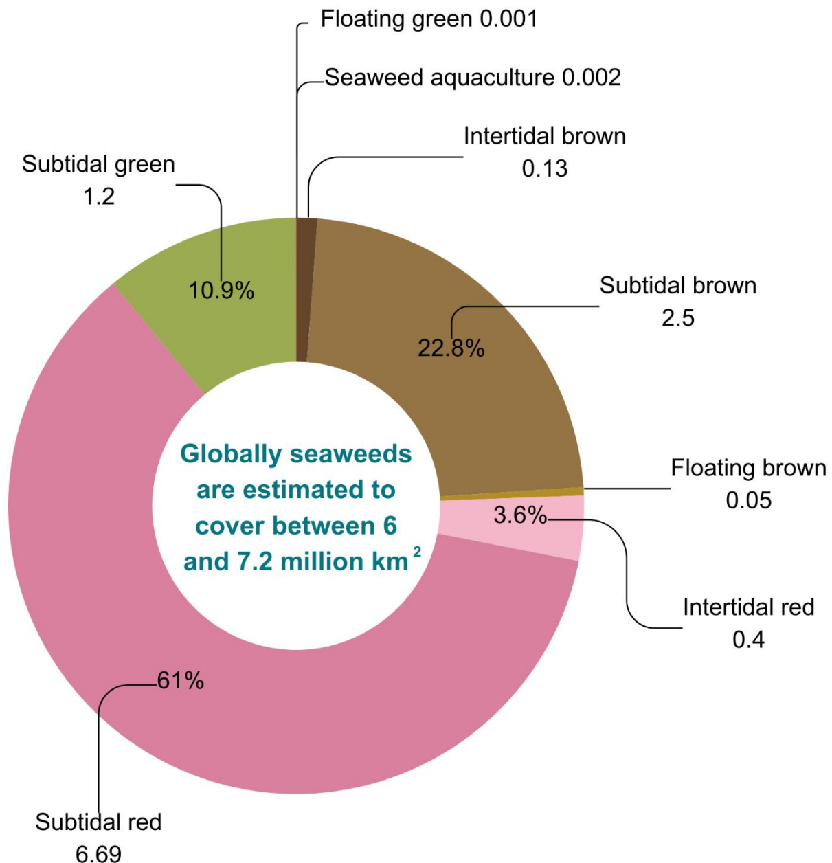
Figure 2. Estimated global area coverage (million km 2 ) by different seaweed groups. Figure adapted from Duarte et al. (2022). Labels show estimated area coverage by seaweed habitat (outside), and percentage contribution of each habitat to estimated total seaweed coverage (inside). Subtidal and intertidal red and brown seaweed area was estimated using a global niche modelling approach (Duarte et al., 2022). Subtidal green value is from McNeil et al. (2016). Floating green value is from Liu et al. (2013a) and Zhang et al. (2019). Floating brown seaweed value is from Wang et al. (2019), Qi et al. (2017) and Zhang et al. (2019).
